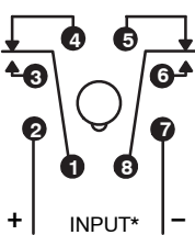
DPDT, 2 Form "C" (8-Pin Type)
